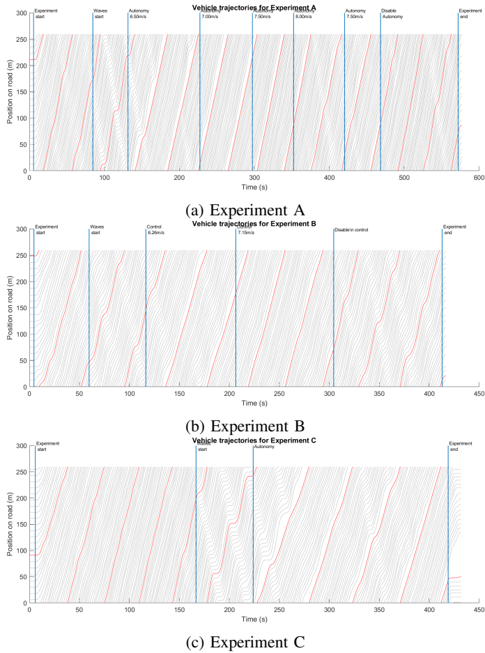
Fig. 5: Vehicle positions over time
